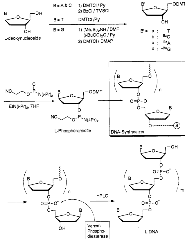
Figure 1. Synthesis of enantio- and meso-DNAs.
